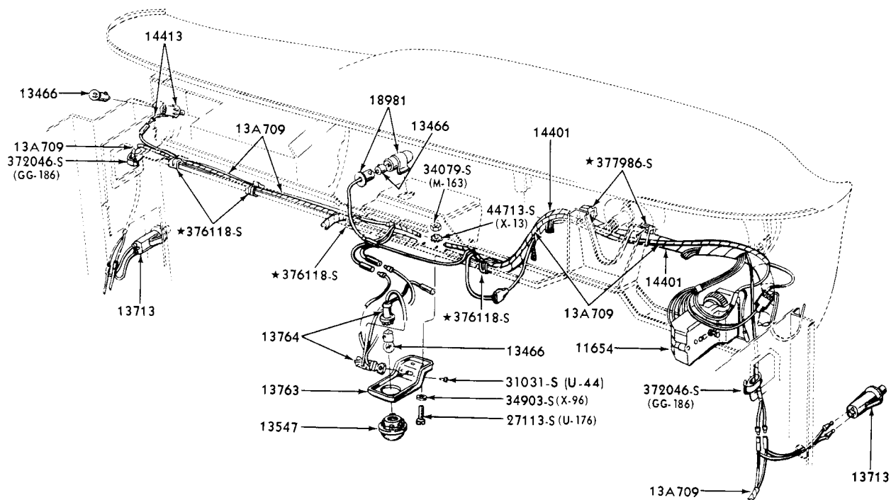
1964/ COURTESY LAMPS & WIRING - INSTRUMENT PANEL (FAIRLANE)
