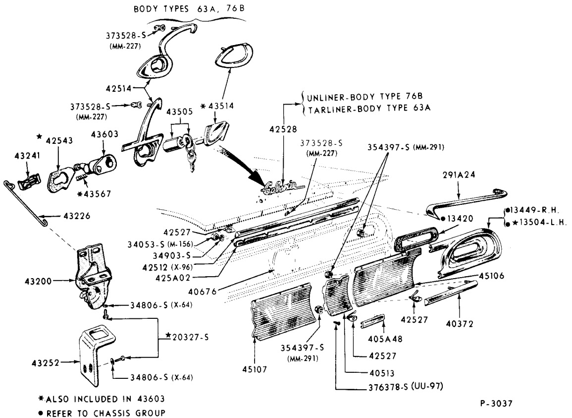
LUGGAGE COMPARTMENT DOOR LATCH, MOULDING and RELATED PARTS 1960 FORD-BODY TYPES 54,62,63,75,76
