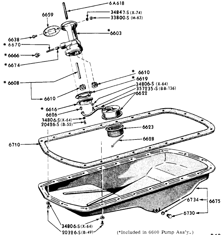
1960/61 OIL PUMP, OIL PAN &amp; RELATED PARTS (6 CYLINDER 223 ENGINE)
