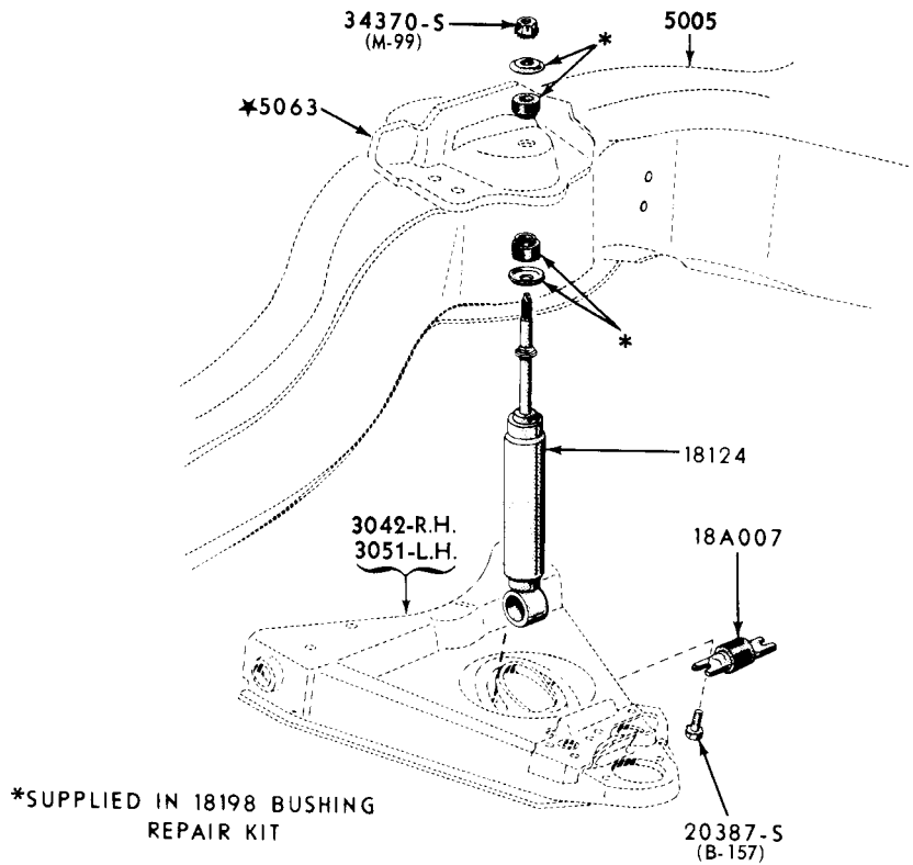
1960 SHOCK ABSORBER-FRONT (THUNDERBIRD)
