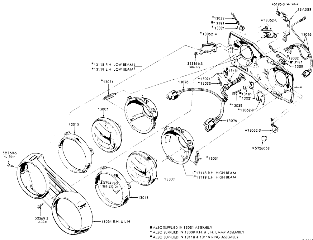
1962 HEADLAMP (FAIRLANE)
