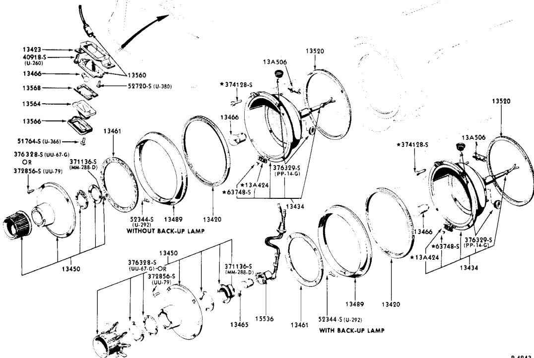
1964 REAR LAMP, BACK UP LAMP & LICENSE PLATE LAMP (FORD-CUSTOM & GALAXIE)
