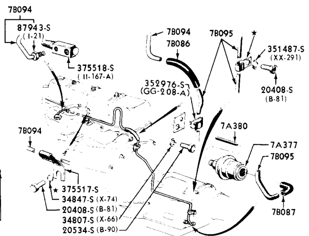
6 CYLINDER 223 &amp; 240 ENGINES
