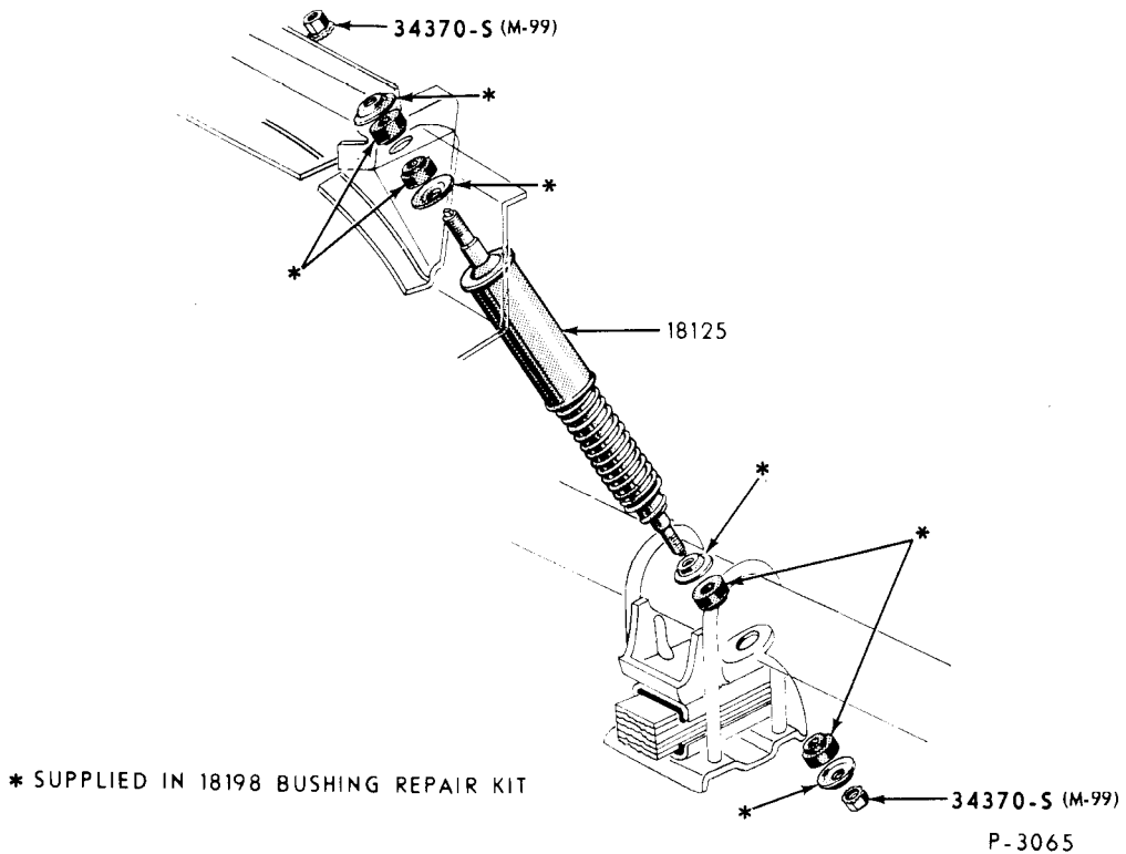
1960 SHOCK ABSORBER-REAR (THUNDERBIRD)
