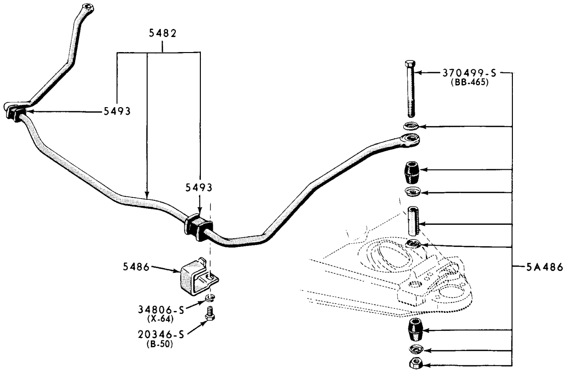
1960 STABILIZER (THUNDERBIRD)-TYPICAL
