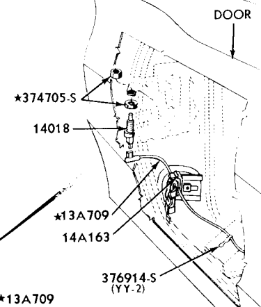
DOOR AJAR WIRING LAMP CONTROL SWITCH INSTALLATION
