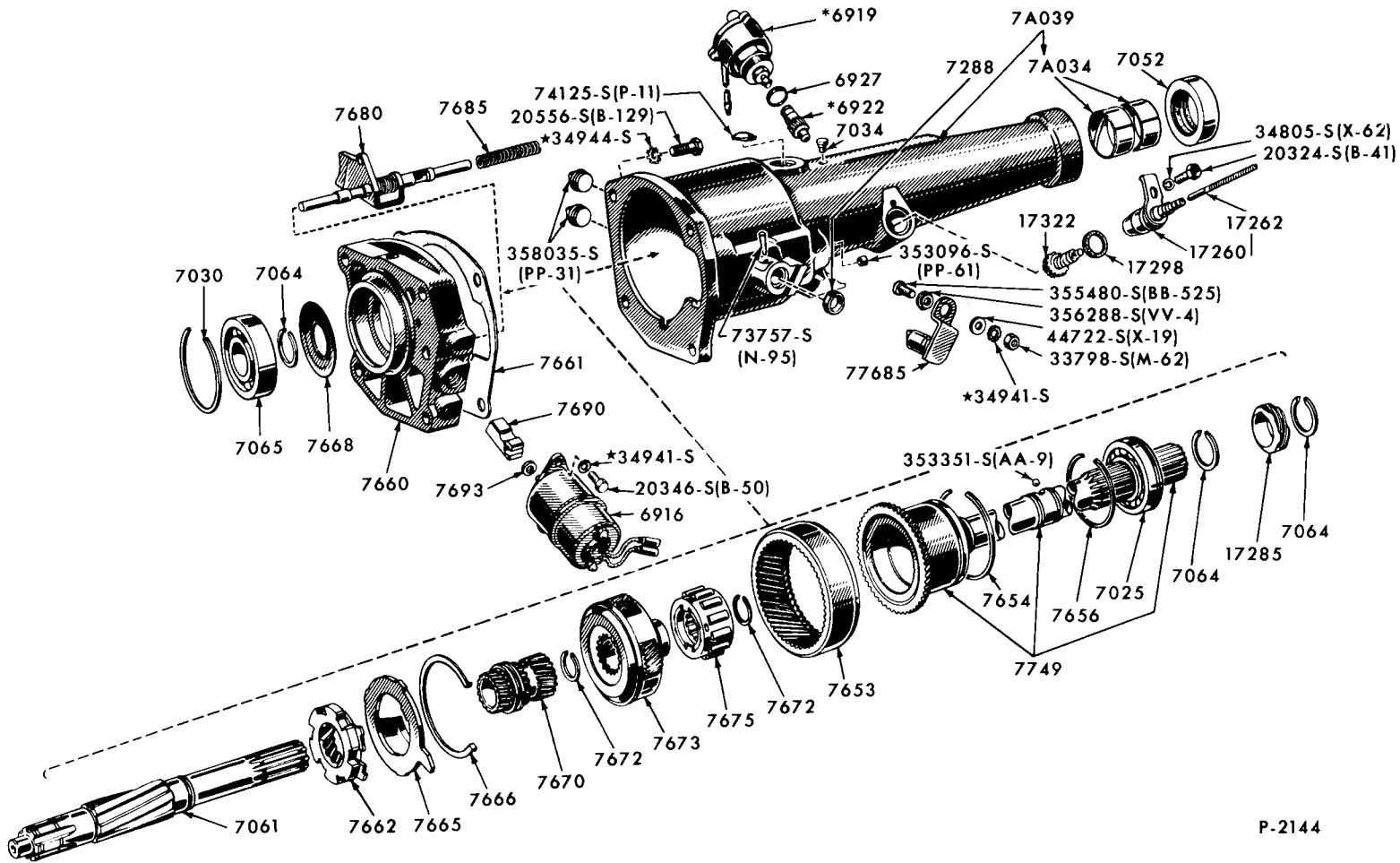
3 SPEED OVERDRIVE TRANSMISSION HOUSING & RELATED PARTS (8 CYLINDER 352, 390 ENGINES)-TYPICAL 1960/ FORD 1960 THUNDERBIRD
