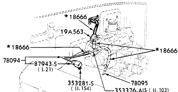
STANDARD BRAKES & CRUISE-O-MATIC TRANSMISSION 352 & 390 C.I.D. ENGINES
