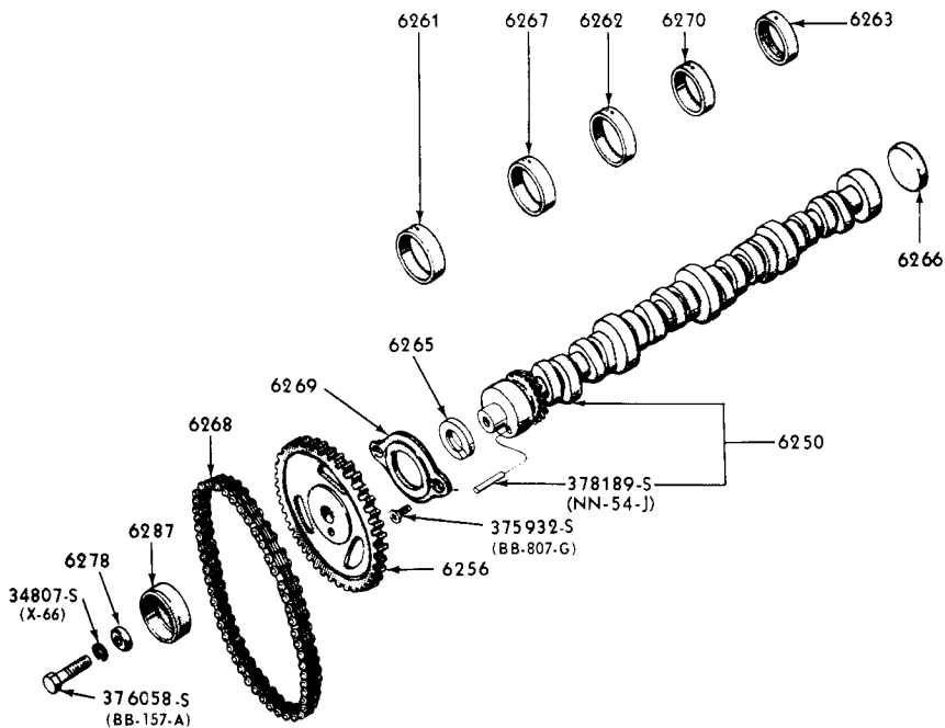
1962/ CAMSHAFT, GEAR, BEARINGS ETC. (8 CYLINDER 221, 260, 289 ENGINES)-TYPICAL
