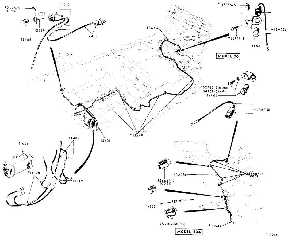
1960 GLOVE &amp; LUGGAGE COMPARTMENT LAMPS &amp; WIRING (THUNDERBIRD)
