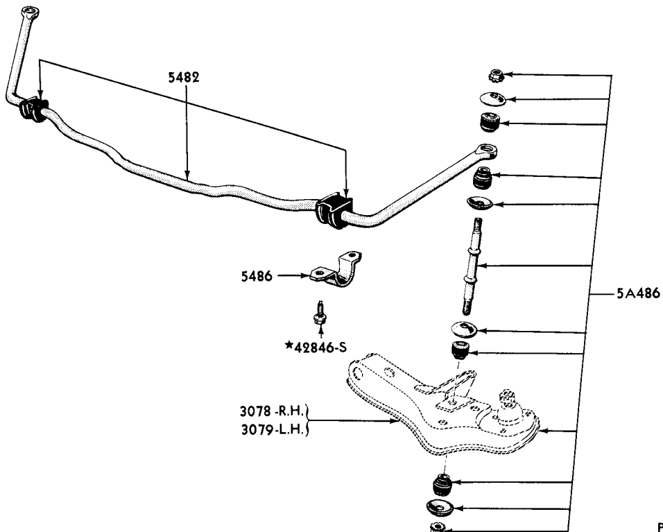
1961/ STABILIZER BAR (THUNDERBIRD)
