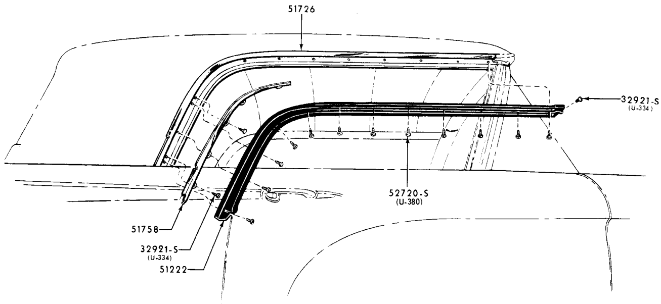
1960 THUNDERBIRD ROOF SIDE RAIL WEATHERSTRIP & RELATED PARTS-BODY TYPE 63
