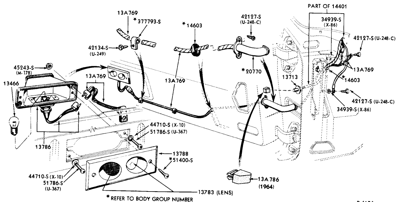
1963/64 COURTESY LAMP &amp; WIRING-INTERIOR DOOR (THUNDERBIRD)
