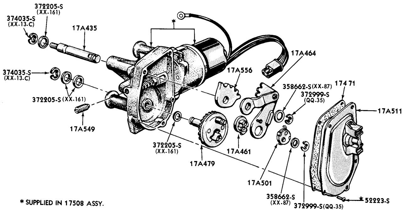
1963/64 WINDSHIELD WIPER (FORD)
