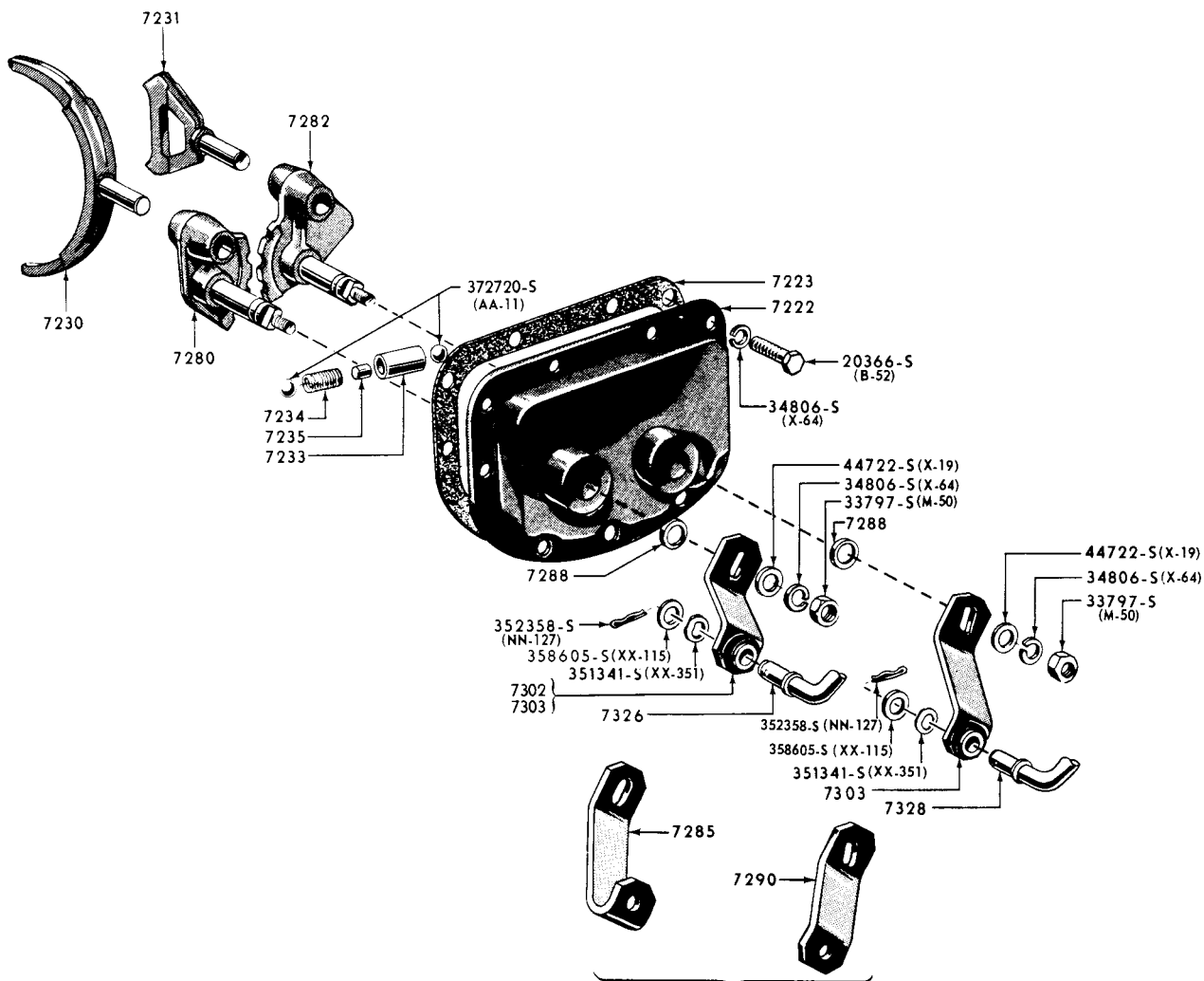
OVERDRIVE TRANSMISSION
