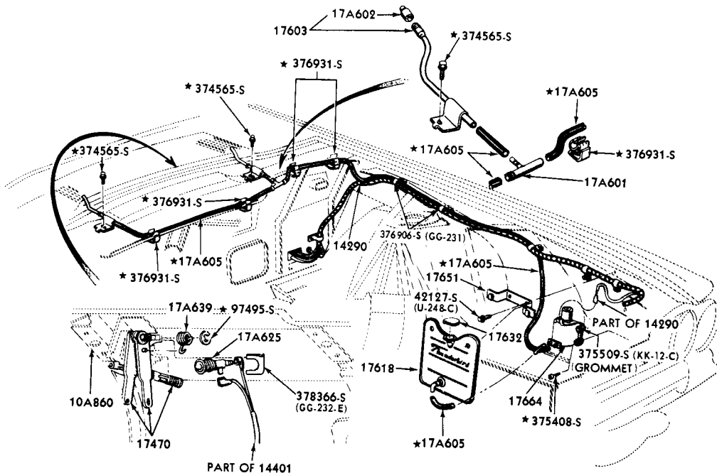
1963/ WINDSHIELD WIPER AND RELATED PARTS - HYDRAULIC (THUNDERBIRD)
