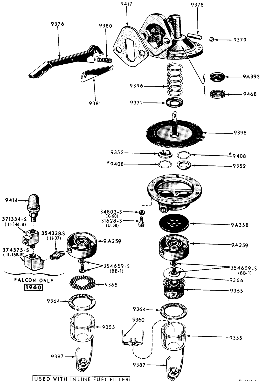
FUEL PUMP (6 & 8 CYLINDER ENGINES)-TYPICAL 1960/61 FORD, FALCON 1960/61 THUNDERBIRD-EXCEPT 430 ENGINES
