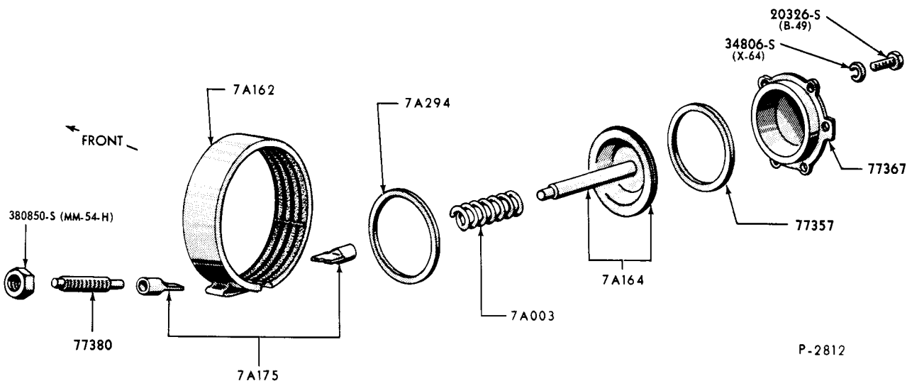
1960/64 REAR SERVO & BAND-FORD, FAIRLANE, FALCON-TYPICAL
