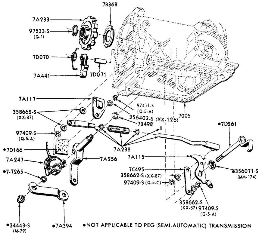
1964/ PARKING PAWL, THROTTLE &amp; MANUAL CONTROL LINKAGE-FORD, FAIRLANE-TYPICAL
