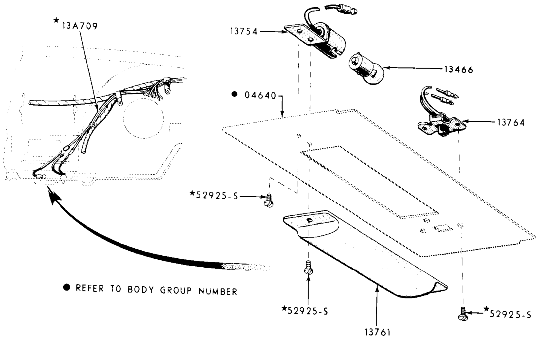
1960 GLOVE &amp; LUGGAGE COMPARTMENT LAMPS &amp; WIRING (THUNDERBIRD)
