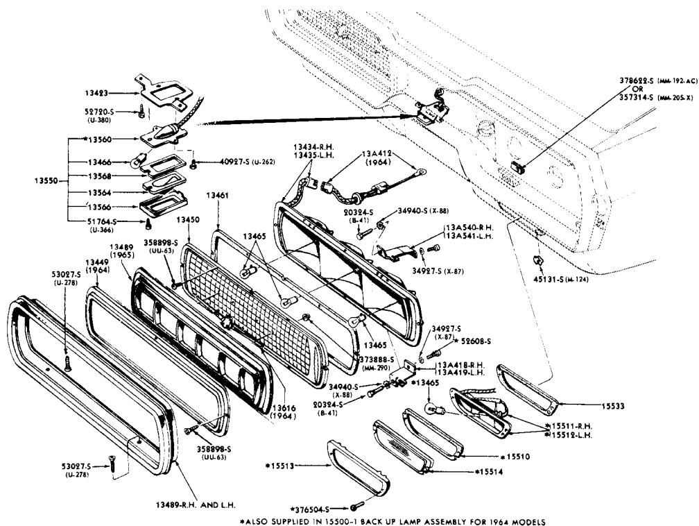
1964/ REAR LAMP, BACK UP LAMP &amp; LICENSE PLATE LAMP (THUNDERBIRD)
