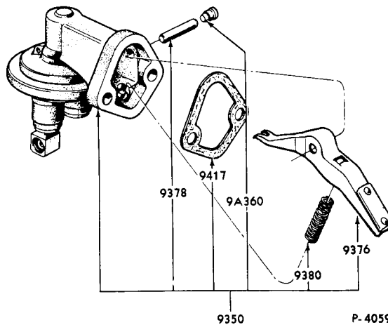
1963 FUEL PUMP (6 CYLINDER 170 ENGINE)-FAIRLANE (CARTER)
