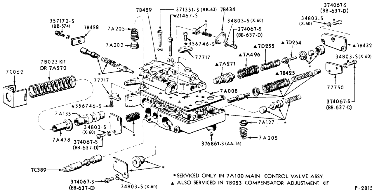
1960/64 MAIN CONTROL VALVE BODY ASSY. -(BASIC 7A100)-FORD, FAIRLANE, FALCON-TYPICAL
