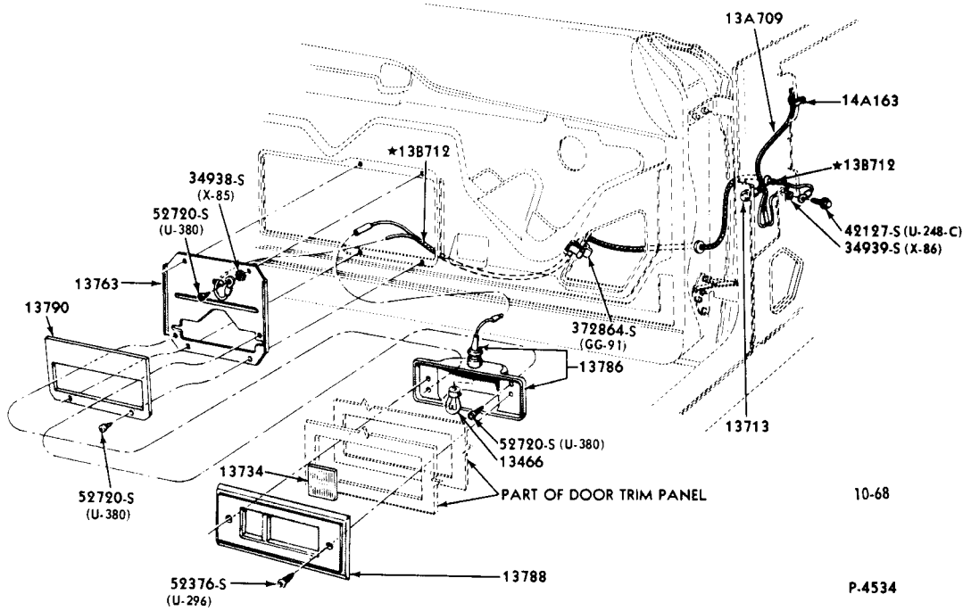
1964/ COURTESY LAMP &amp; WIRING-INTERIOR DOOR (FAIRLANE)
