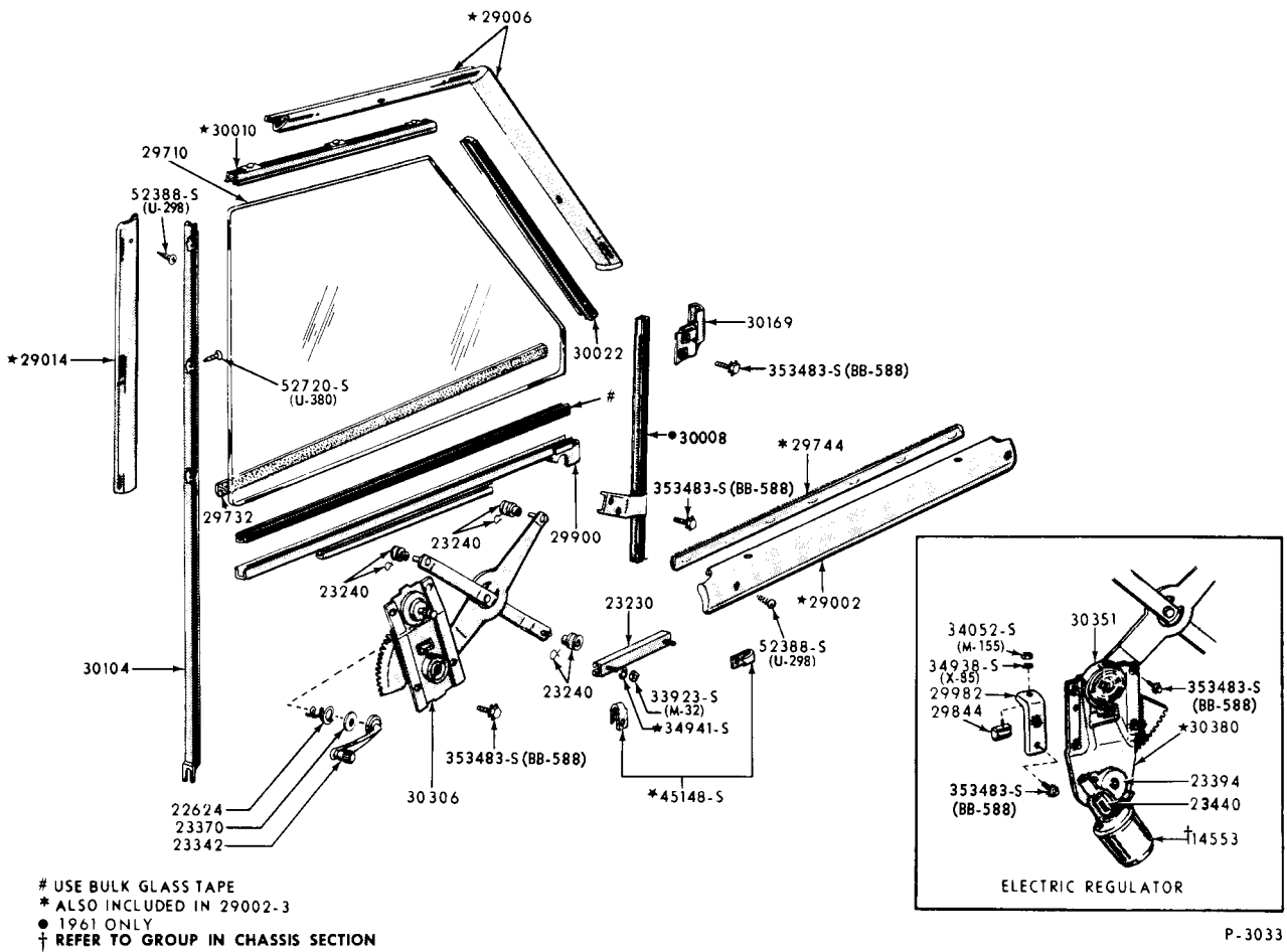
1960/61 FRONT QUARTER WINDOW PARTS -BODY TYPE A(59C)
