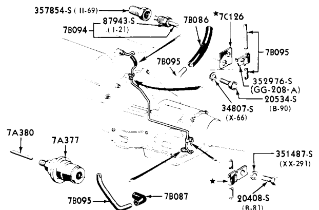
8 CYLINDER 292 ENGINE WITH F/M/2 TRANSMISSION
