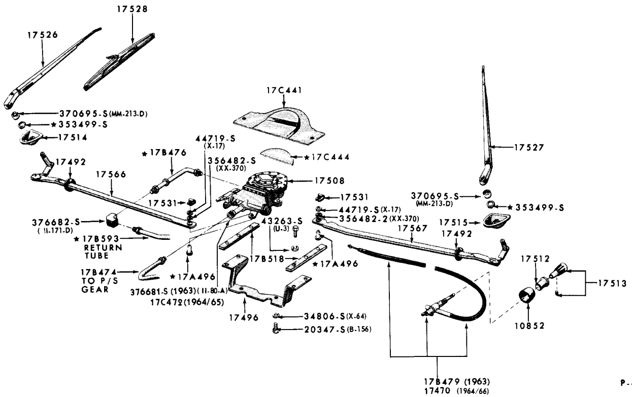
1963/ WINDSHIELD WIPER AND RELATED PARTS - HYDRAULIC (THUNDERBIRD)
