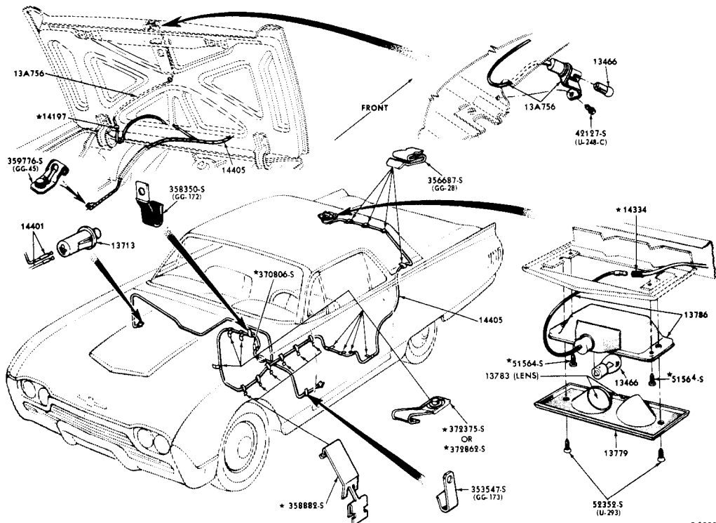
1961/63 DOME LAMP & LUGGAGE COMPARTMENT LAMP (THUNDERBIRD 63A)
