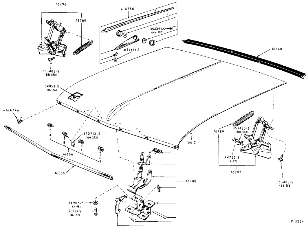
1961 HOOD and RELATED PARTS (FORD)
