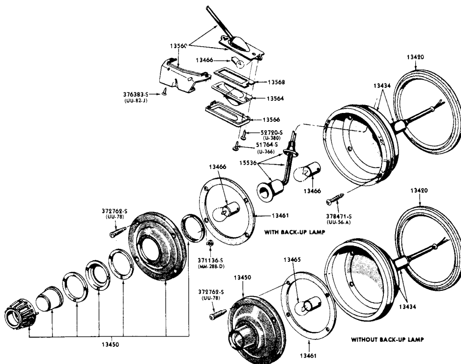
1964 REAR LAMP, BACK UP LAMP &amp; LICENSE PLATE LAMP (FALCON)
