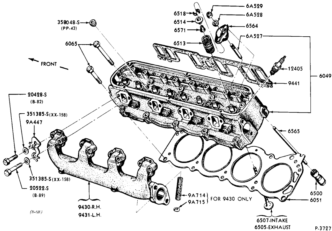
1962/ CYLINDER HEAD, VALVES, EXHAUST MANIFOLDS (8 CYLINDER 221, 260, 289 ENGINES)-TYPICAL
