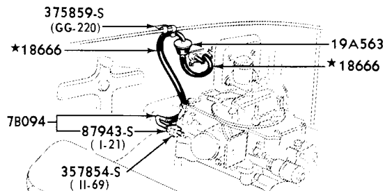
STANDARD BRAKES & STANDARD TRANSMISSION 292 C.I.D. ENGINE
