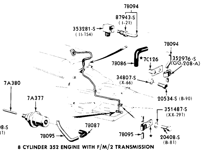
8 CYLINDER 352 ENGINE WITH F/M/2 TRANSMISSION
