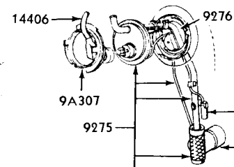
FUEL TANK SENDER (LOW FUEL UNIT)
