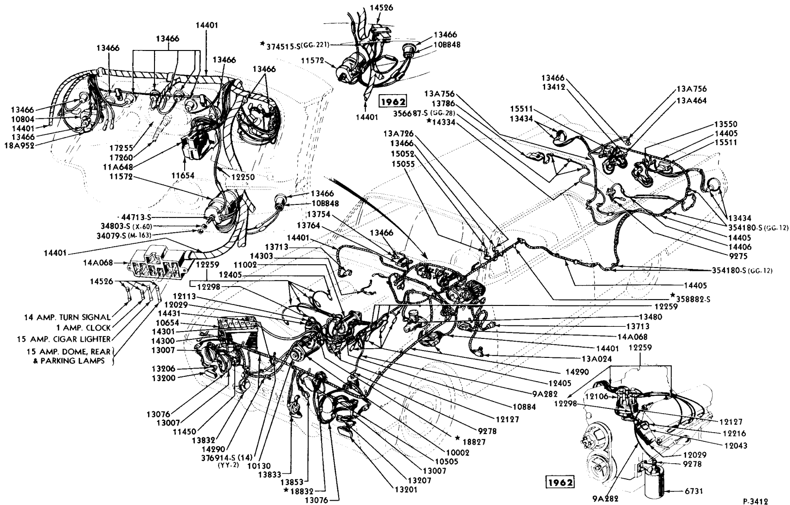
1961/62 WIRING SYSTEM (THUNDERBIRD)-TYPICAL
