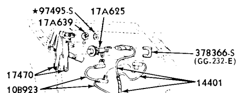
R.H. COWL SIDE PANEL WIRING & FLASHER INSTALLATION
