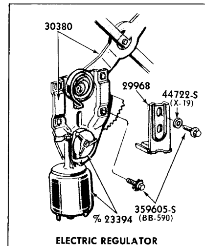
ELECTRIC REGULATOR
