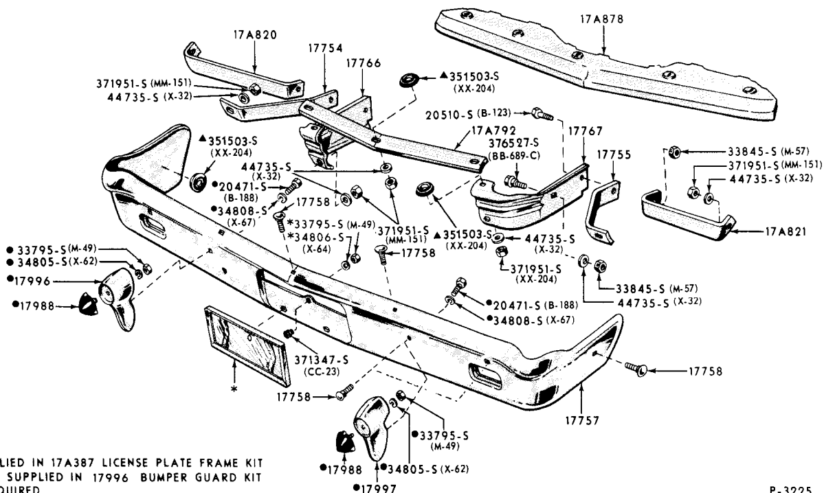
FRONT BUMPER and RELATED PARTS
