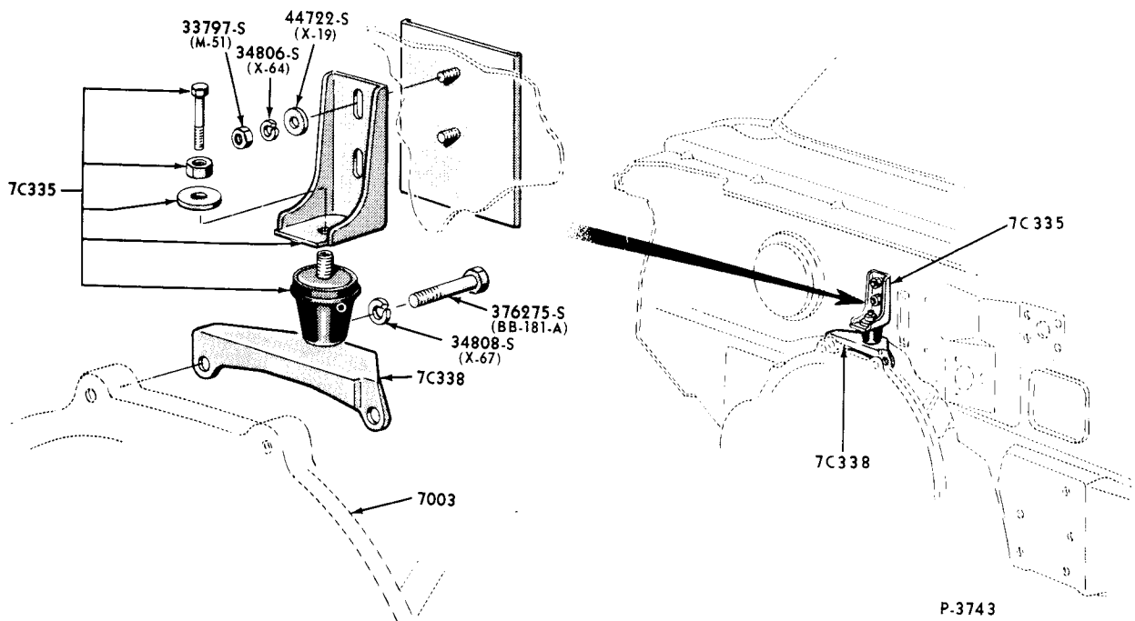
1962 C/M TRANSMISSION DASH PANEL INSULATOR &amp; BRACKET TO TRANSMISSION-THUNDERBIRD-TYPICAL
