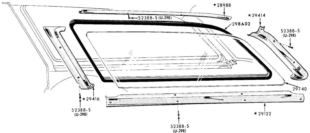
1960/61 FRONT QUARTER WINDOW PARTS -BODY TYPE A(59C)
