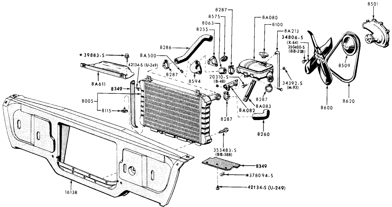
1960/63 COOLING SYSTEM (FORD-CUSTOM &amp; GALAXIE) -6 CYL, 223
