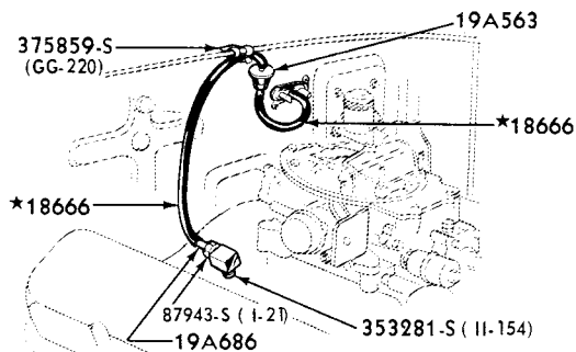
STANDARD BRAKES & STANDARD TRANSMISSION 352 & 390 C.I.D. ENGINES
