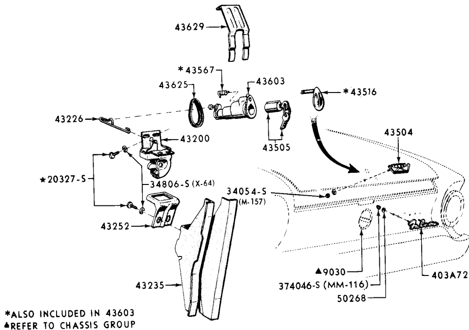
LUGGAGE COMPARTMENT DOOR LOCK and RELATED PARTS 1960/61 FALCON - BODY TYPES 58A, 64A
