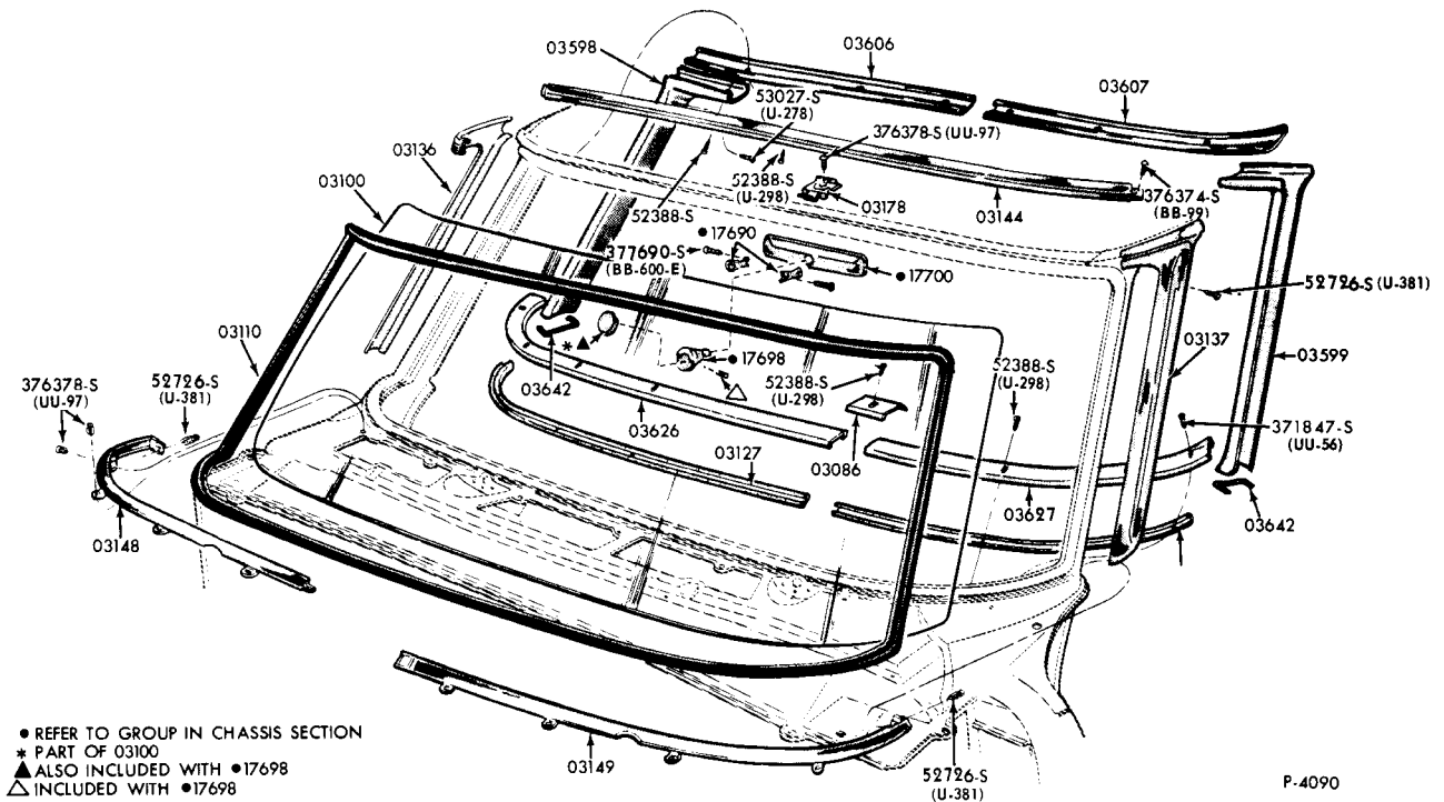
1963/64 FORD WINDSHIELD PARTS - BODY TYPES A(57, 63)
