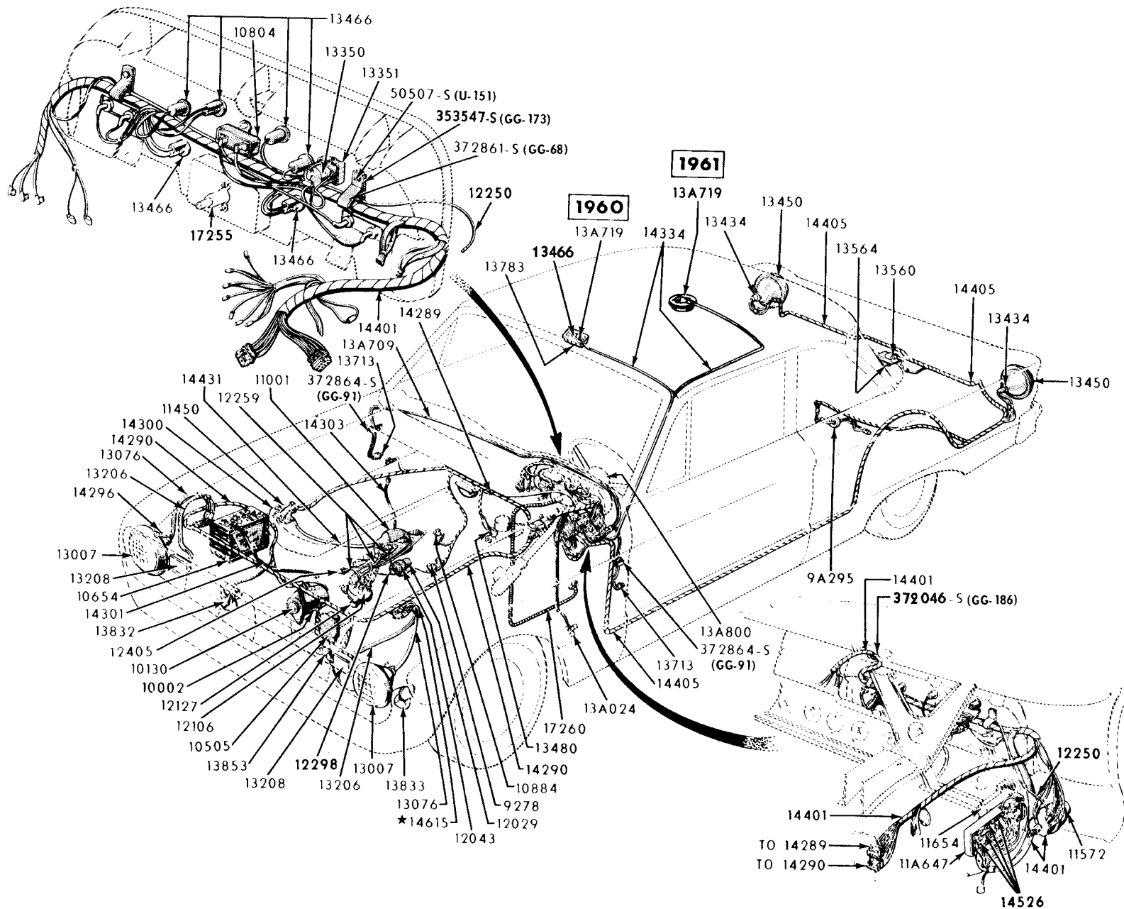
1960/62 WIRING SYSTEM (FALCON)
