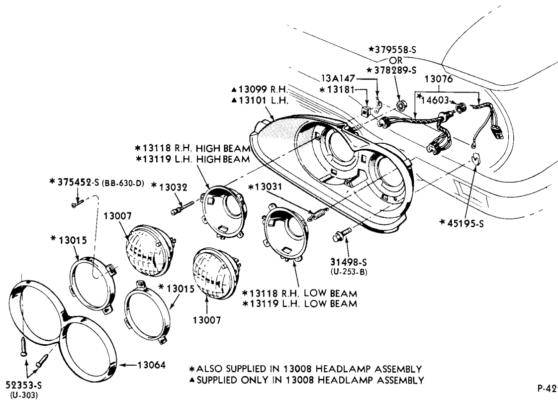
1964/ HEADLAMP (THUNDERBIRD)
