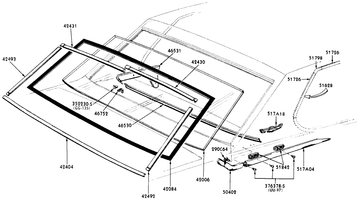
1964 BACK WINDOW &amp; RELATED PARTS - BODY TYPE A(54)
