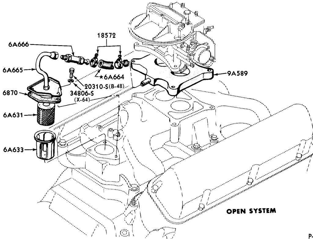
1962/ CRANKCASE VENT SYSTEM-INTAKE MANIFOLD TYPE-EMISSION REDUCTION (8 CYLINDER 221, 260, 289 ENGINES)
