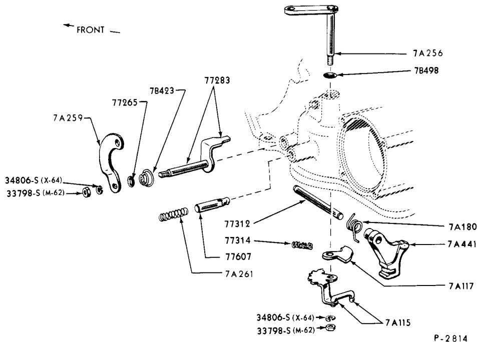
1960/64 PARKING PAWL, THROTTLE &amp; MANUAL CONTROL LINKAGE-FORD, FAIRLANE, FALCON-TYPICAL
