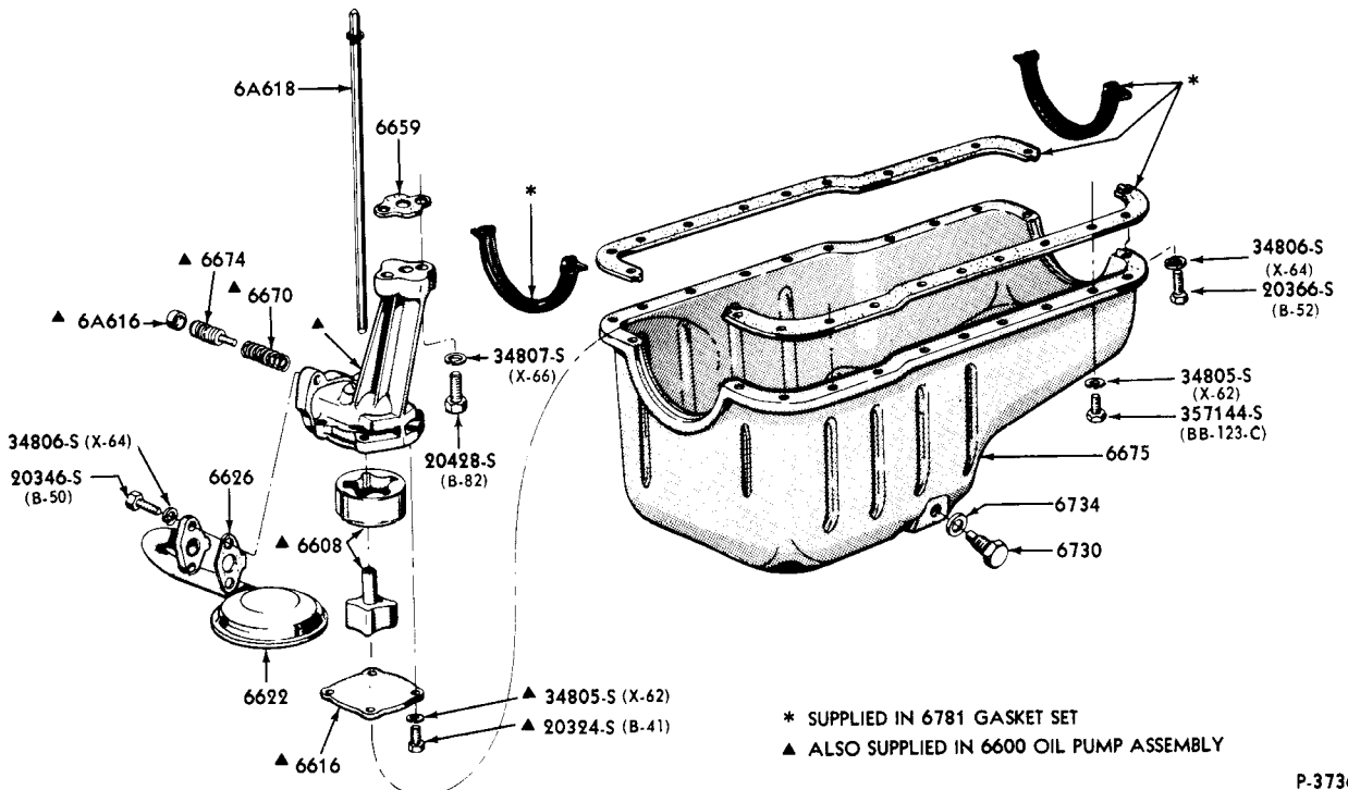
1962/ OIL PUMP, OIL PAN &amp; RELATED PARTS (8 CYLINDER 221, 260, 289 ENGINES)-TYPICAL
