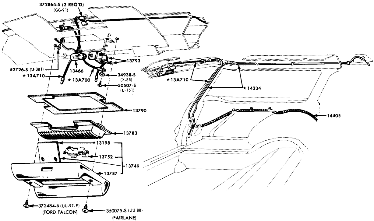
CARGO AREA LAMP (STATION WAGON) 1964 FORD 1964/ FAIRLANE & FALCON
