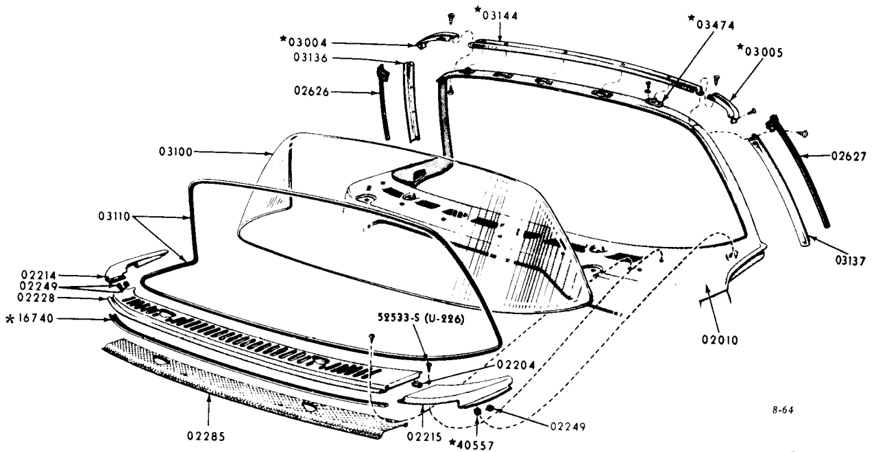
1960 THUNDERBIRD WINDSHIELD PARTS - BODY TYPE S(63A)
