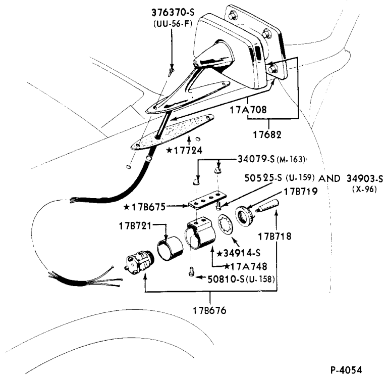
1963 REMOTE CONTROL REAR VIEW MIRROR-FENDER MOUNTED (FAIRLANE, FALCON, FORD)
