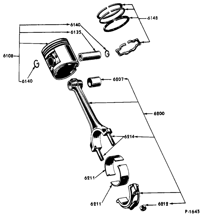
1960/64 PISTON &amp; CONNECTING ROD (6 CYL. 223 &amp; 8 CYL. 292 ENGINES)-TYPICAL
