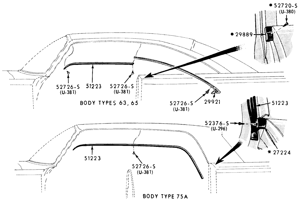
1960 THUNDERBIRD ROOF SIDE RAIL WEATHERSTRIP & RELATED PARTS-BODY TYPE 63
