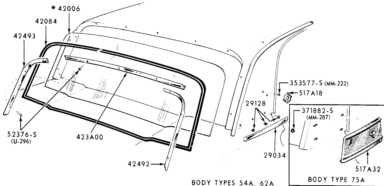
1960 BACK WINDOW & RELATED PARTS - BODY TYPES A (54A, 62A, 75A)
