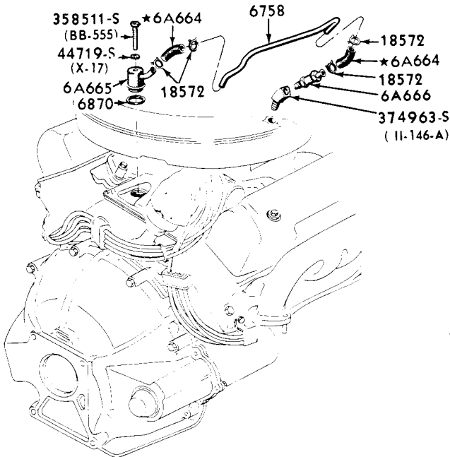
8 CYL. 292 ENGINE EMISSION REDUCTION CONTROL (1961/62)
