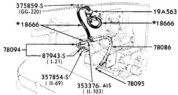
STANDARD BRAKES & FORDOMATIC-2 SPEED-TRANSMISSION 292 C.I.D. ENGINE
