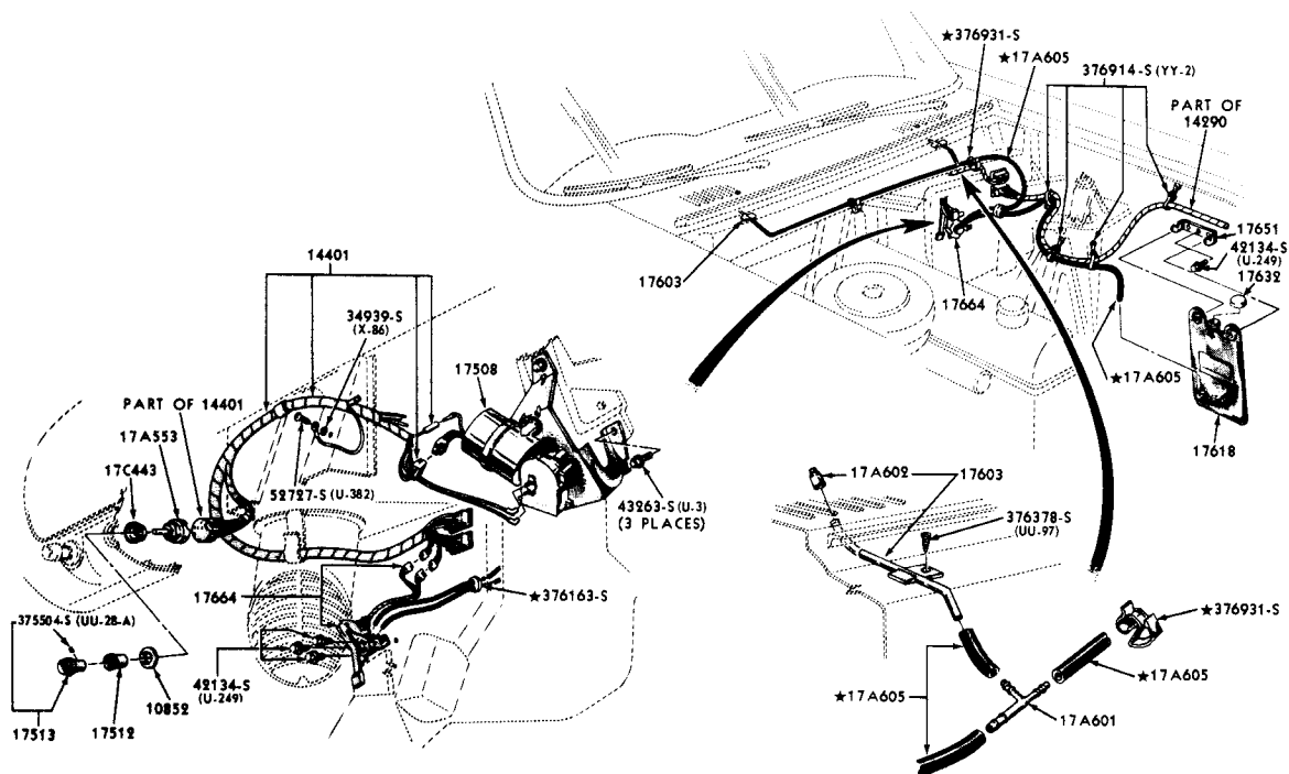
1933/ WINDSHIELD WIPER (FALCON)
