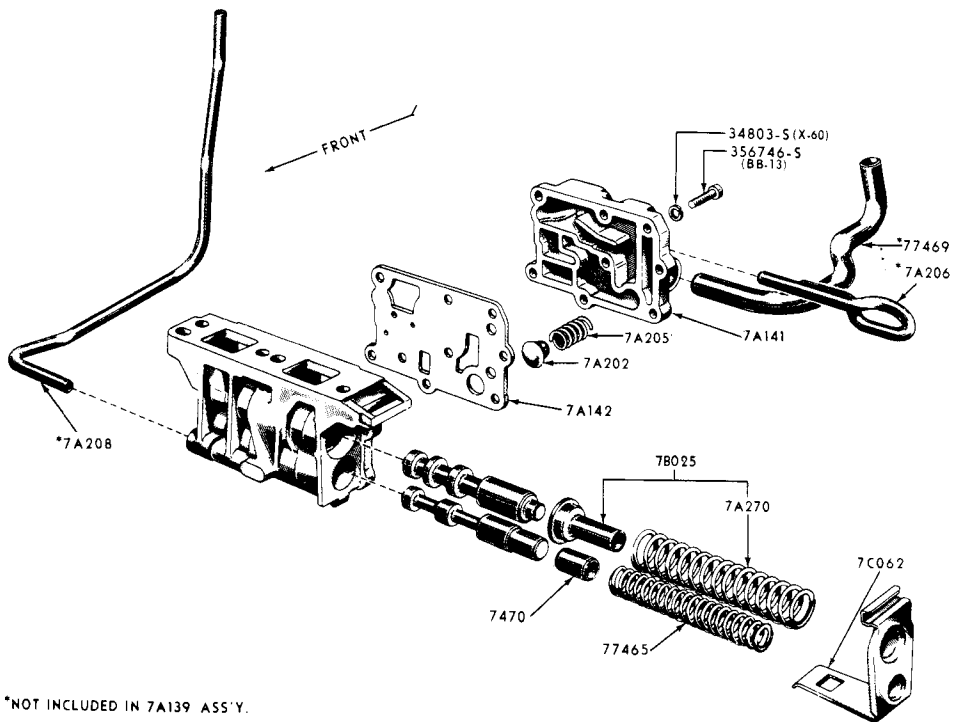
1960/ OIL PRESSURE REGULATOR &amp; RELATED PARTS-(BASIC 7A139)-FORD, THUNDERBIRD-TYPICAL
