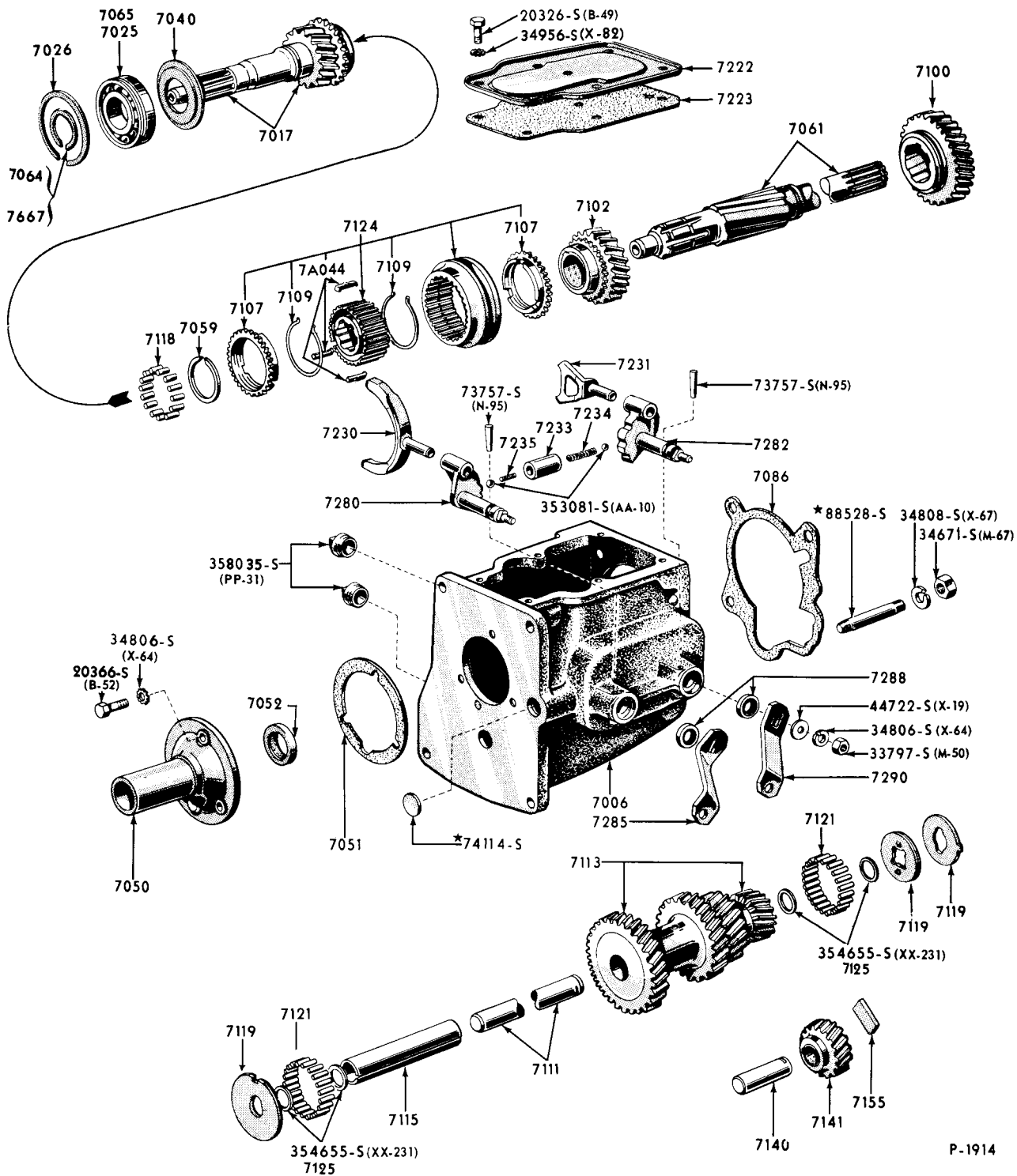
1960/ 3 SPEED OVERDRIVE TRANSMISSION-LESS HOUSING (6 & 8 CYLINDER 223, 289, 292 ENGINES)-FORD, FAIRLANE-TYPICAL
